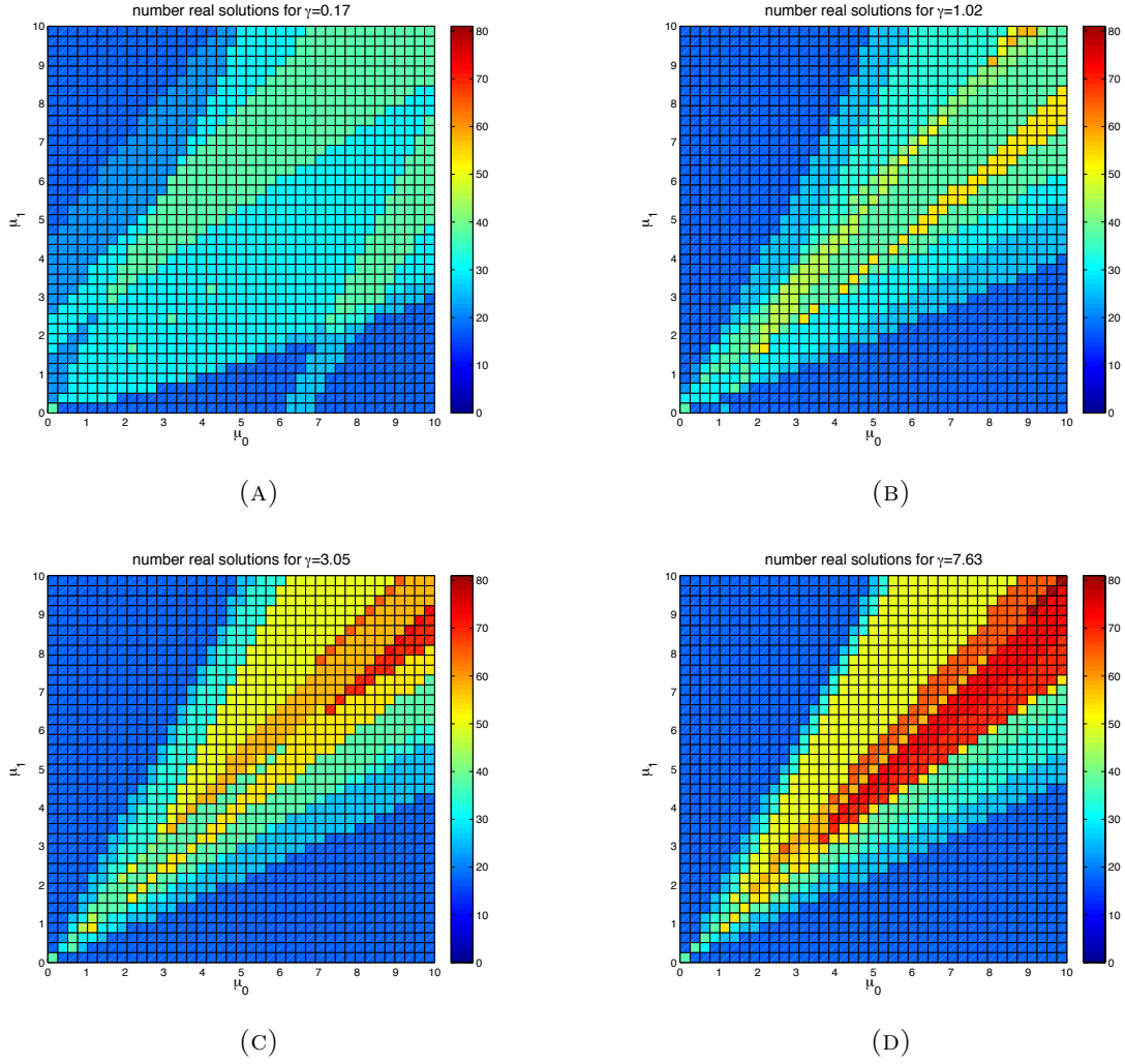
FIGURE 4. Regions with various numbers of real solutions to the Monks equations in parameter space (\mu_0, \mu_1, \gamma) . The displayed region is for (\mu_0, \mu_1) \in [0, 10] \times [0, 10] . At \gamma = 0 there is one solution everywhere, namely the 0 solution; this plot omitted. For low \gamma , there are few solutions near the parameter-origin, as in (a). As \gamma increases, regions of higher numbers of solutions appear, and these regions move toward the origin.
