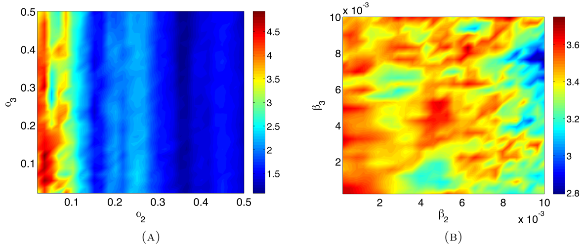
FIGURE 19. Phase diagram for ILM detectability at defected pillar in 50-pillar crystal array. Coupling parameters \alpha_2 and \alpha_3 are examined in the left, \beta_2 and \beta_3 in the right. Red areas denotes strong ILM formation whereas blue indicates practically no spontaneously forming ILMs present in the system.
