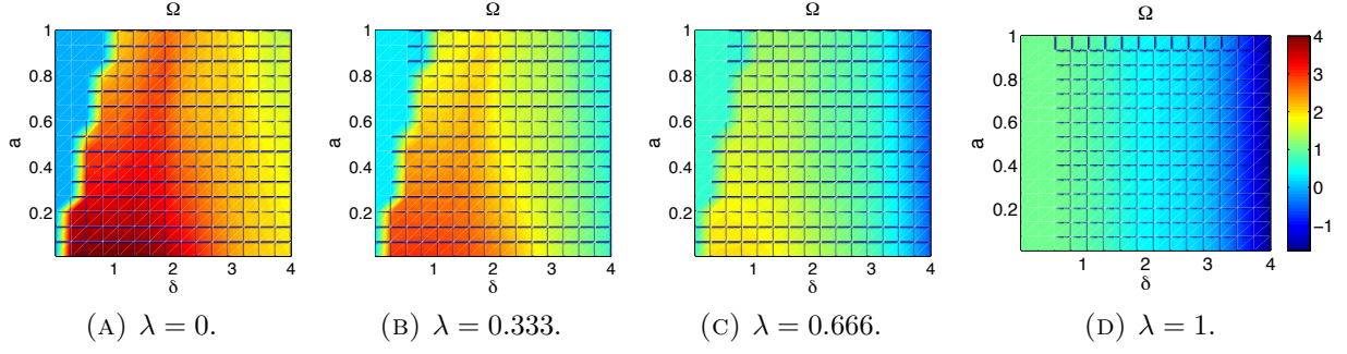
FIGURE 27. Objective function contours for a grid of (\delta, a) pairs for 2D cooperating robots, with the broken robot being grasped on the first link.
