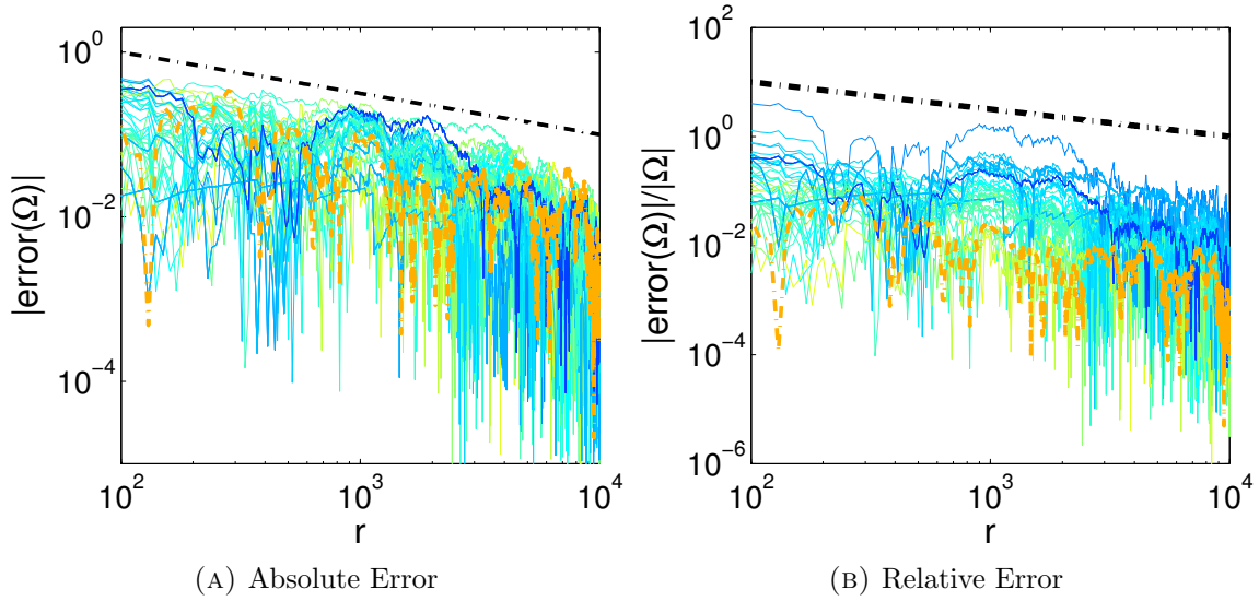
FIGURE 25. Error estimate of \Omega for a host of 3D configurations with varying (\delta, a) as a function of the number of sampling points r . The dashed straight line shows -1/2 power law, which is a typical upper bound for a Monte Carlo based method. The colors in this plot correspond to the \Omega values appearing in Figure 29(b). Blue lines have low \Omega value, and hence, a low number of samples are in the corresponding workspace; high variation in absolute error occurs for these lines, and relative error is higher. In contrast, the thicker orange line is computed from many points, absolute error fluctuates less, and the relative error is lower.
