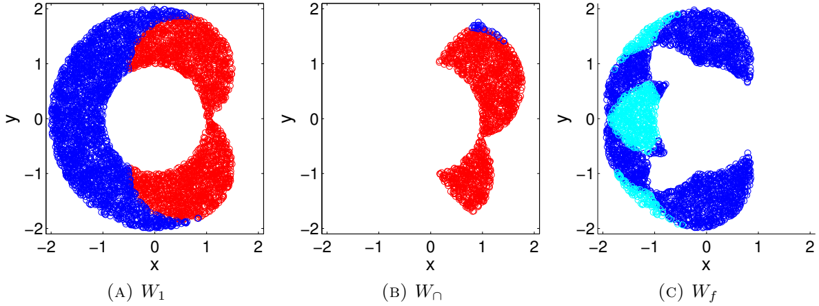
FIGURE 26. Examples of joint-limited workspaces, for \delta = 1.87 , a = 1 , and grasping on the first link, rotated relative to one another. Red indicates a point having one solution, blue indicates two, and cyan indicates four.
