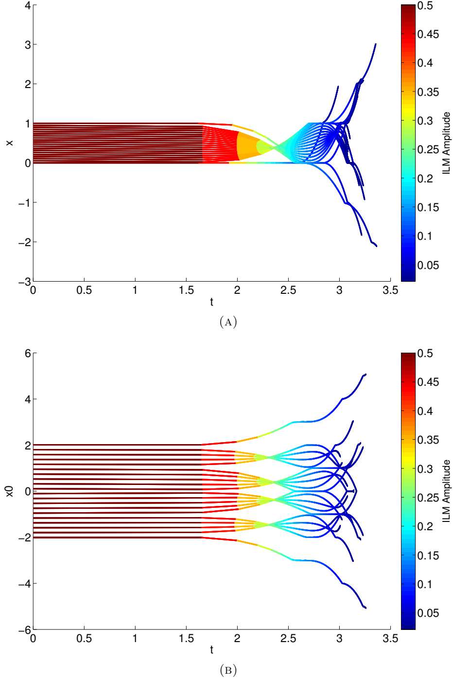
FIGURE 21. Four-variable reduced system, simulations of 20 initial conditions. (a): In the absence of defect, the interval of initial conditions between x_0 = 0 and 1 would be perfectly symmetrical; in this plot, a -5% defect at pillar 0 causes a breaking in symmetry. ILMs are pulled towards the defect, but reflect and bounce. (b): This plot demonstrates a -5% defect, again at pillar 0. This plot would be periodic in x_0 , but placing the defect breaks this, and the only symmetry is reflection across the defected pillar.
