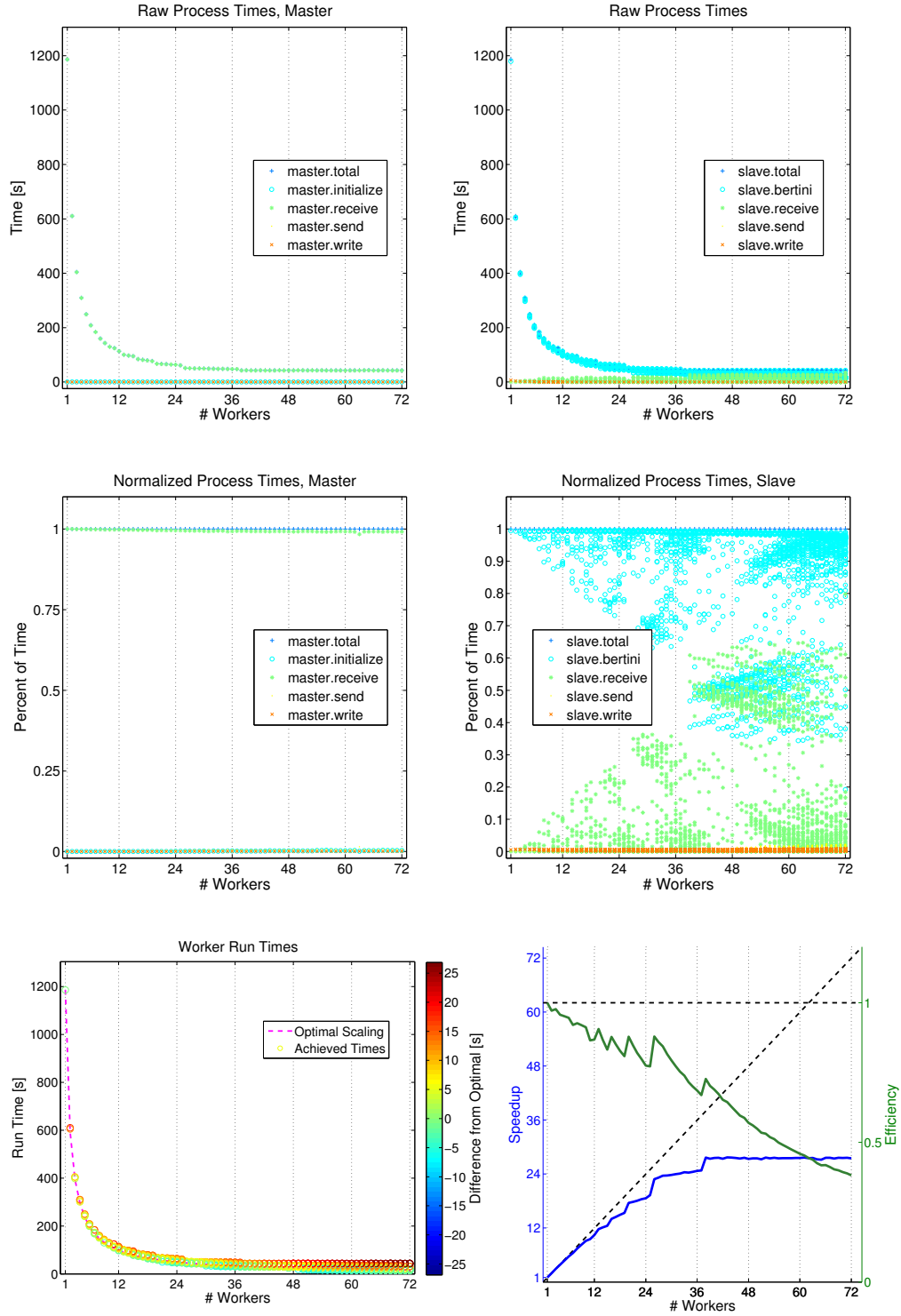
FIGURE 3. Monks equations timing, 8000 parameter points, scaling from 1 to 72 workers. Maximum speedup of \approx 30\times achieved. The relatively small parameter point sample hinders effective distribution of work.
