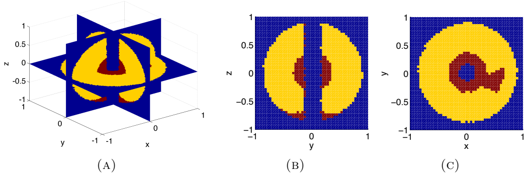
FIGURE 28. Top: Slices of the pre-failure PUMA workspace W_1 by the planes x = 0 (b) and z = 0 (c). (a): Combined picture of workspace with three slices x = 0 , y = 0 , z = 0 . Yellow color: areas accessible the angles satisfying joint limits given in Table 3. Red color: real solutions violating joint limits. Dark blue region: inaccessible.
