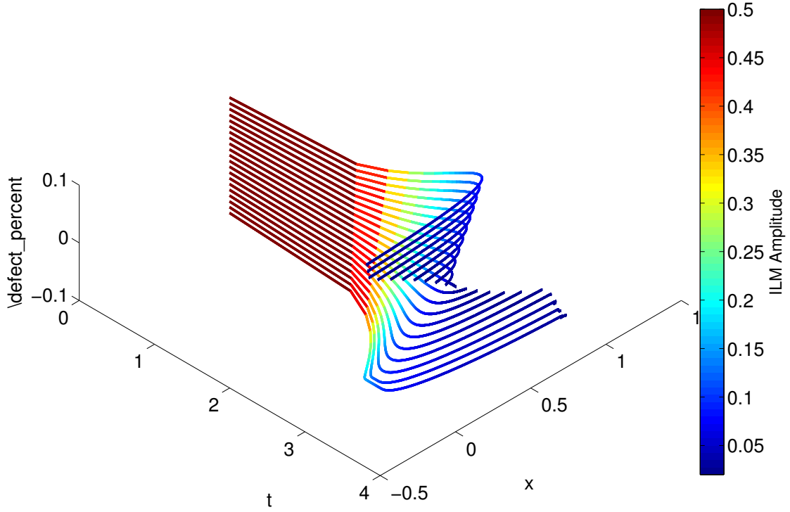
FIGURE 22. Four-variable simulations of reduced ILM dynamics. The color of the lines indicates ILM amplitude. In the vertical axis is an exploration of defect amplitude for the linear restorative parameter, \alpha_1 . Each simulation started from the same point on the array, exactly half way between a normal pillar and one with a defect, at x_0 = 0.5 . With negative perturbations, the ILM is attracted to the defect, but eventually pins to the normal pillar. Positive perturbations cause the opposite effect.
