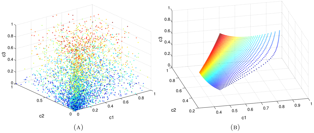
FIGURE 13. Craciun, Helton, Williams, Example 2.2. Each parameter combination yields a unique equilibrium in the unit cube. (a) Random sampling solution set. (b) Mesh solution set. Coloring is determined by the value of (p6 + c3) .
