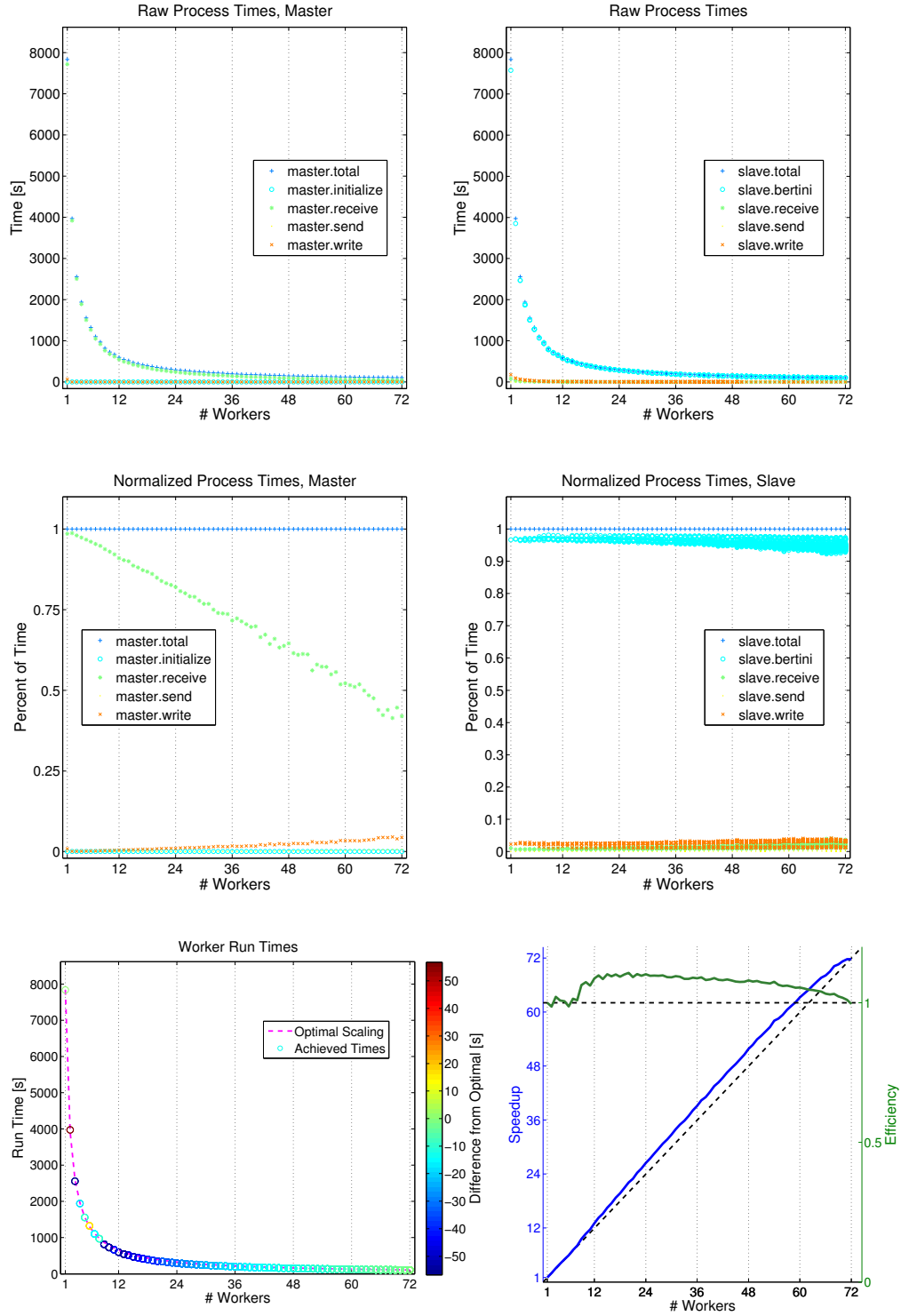
FIGURE 7. Duffing 9 \times 9 timing data. Peak speedup of about 72\times , with 72 processors. Greater than unity efficiency achieved. Peak rate of almost 27400 paths per second.
