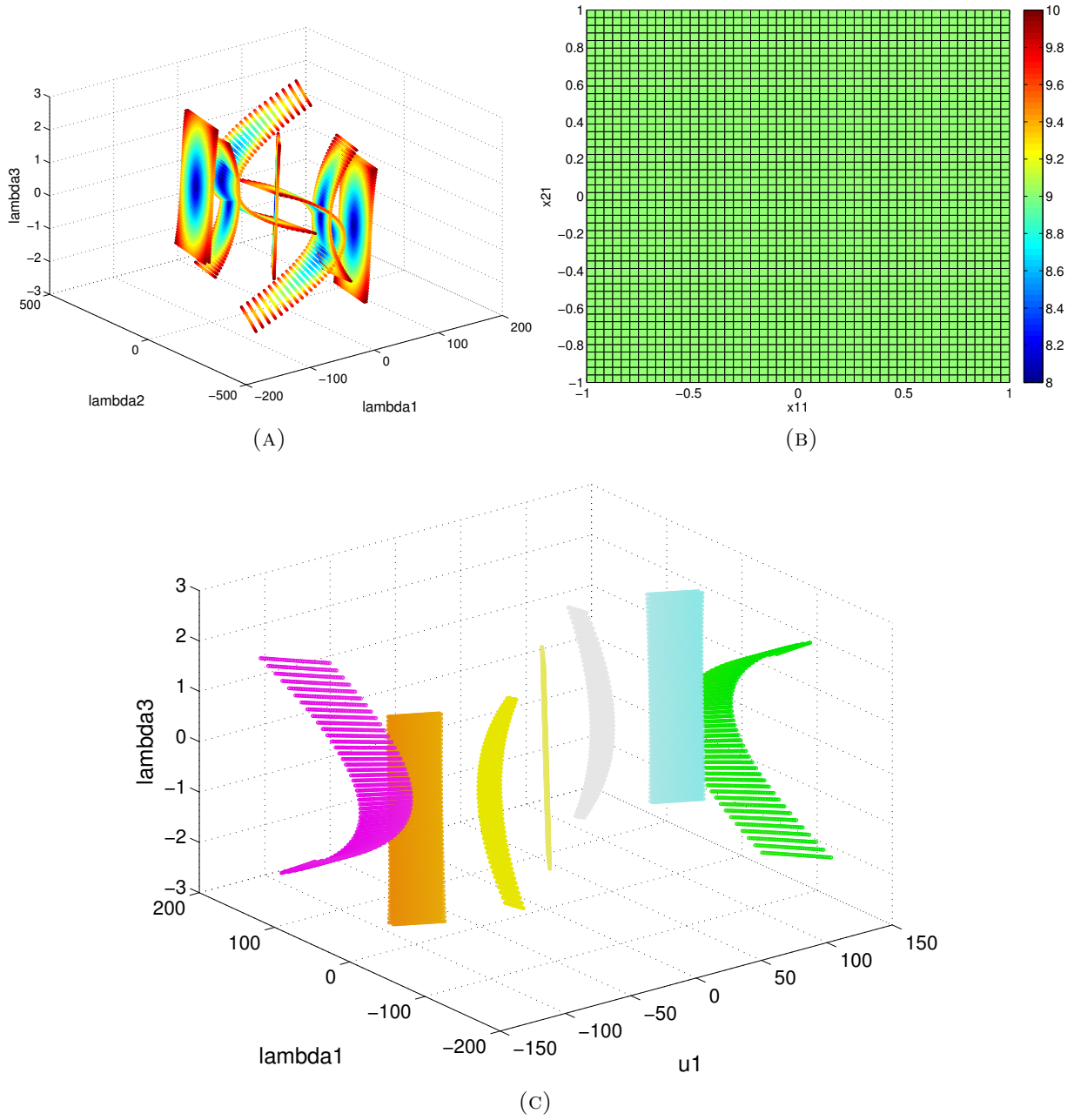
FIGURE 11. Duffing 18 \times 18 solution plots. (a) Projection of solutions onto coordinates (\lambda_1, \lambda_2, \lambda_3) , with color determined by corresponding parameter distance to the origin. (b) The parameter space uniformly has nine real solutions. (c) Projection onto (\lambda_1, u_1, \lambda_3) , with RGB value determined by a triple composed of normalized values of (\mu_3, \mu_4, x_{23})
