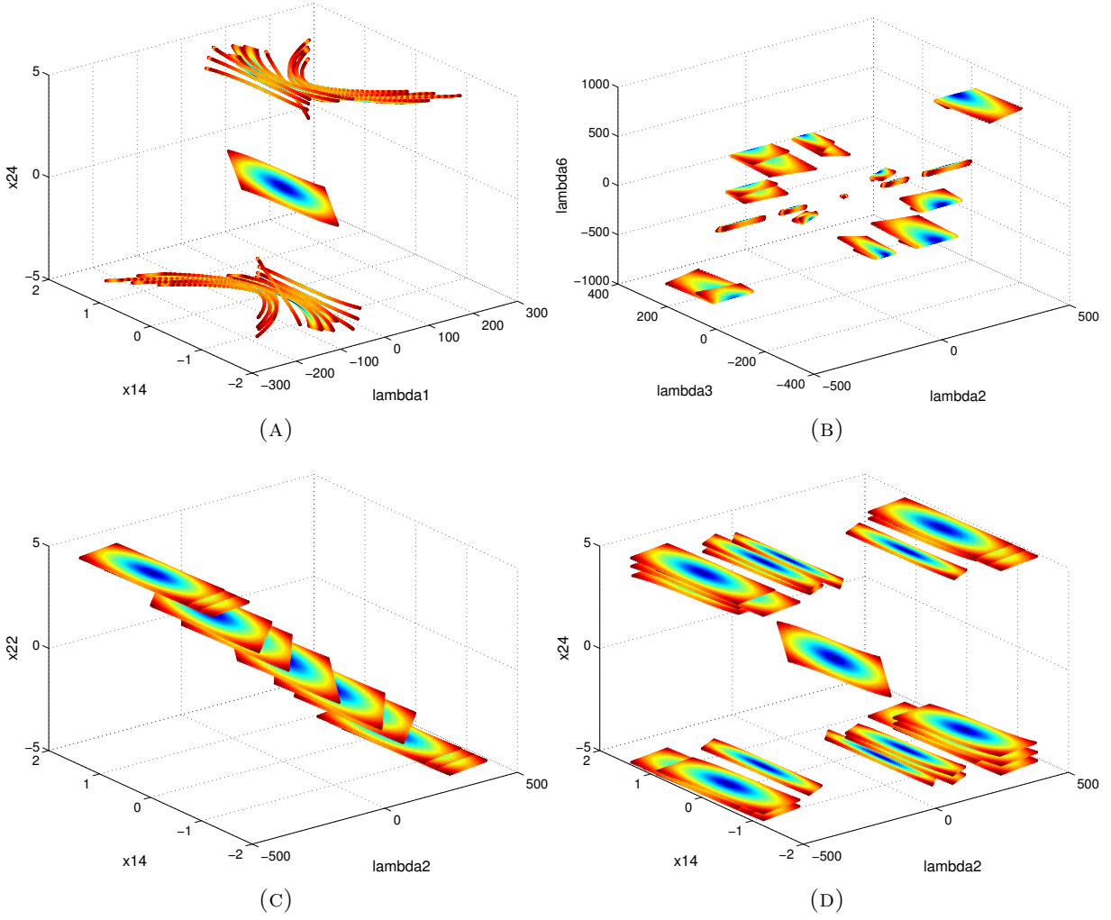
FIGURE 12. Projections of the Duffing 27 \times 27 system onto various combinations of variables. In all four plots shown here, colors of points correspond to the distance to the parameter point from the origin. The system generically has 27 nonsingular finite solutions at each point in parameter space.
