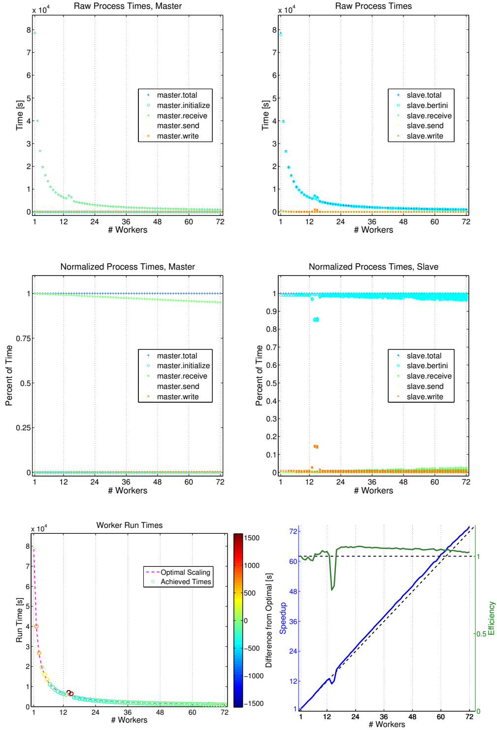
FIGURE 10. Duffing 18 \times 18 timing results. Linear speedup achieved throughout the range of processors used. The small blip at 13 processors indicates another process was using the hard drive, inhibiting Paramotopy performance.
