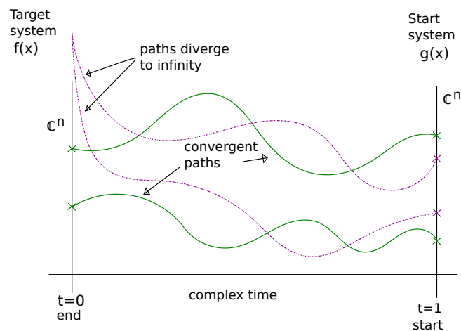
FIGURE 30. Generic Homotopy Continuation
