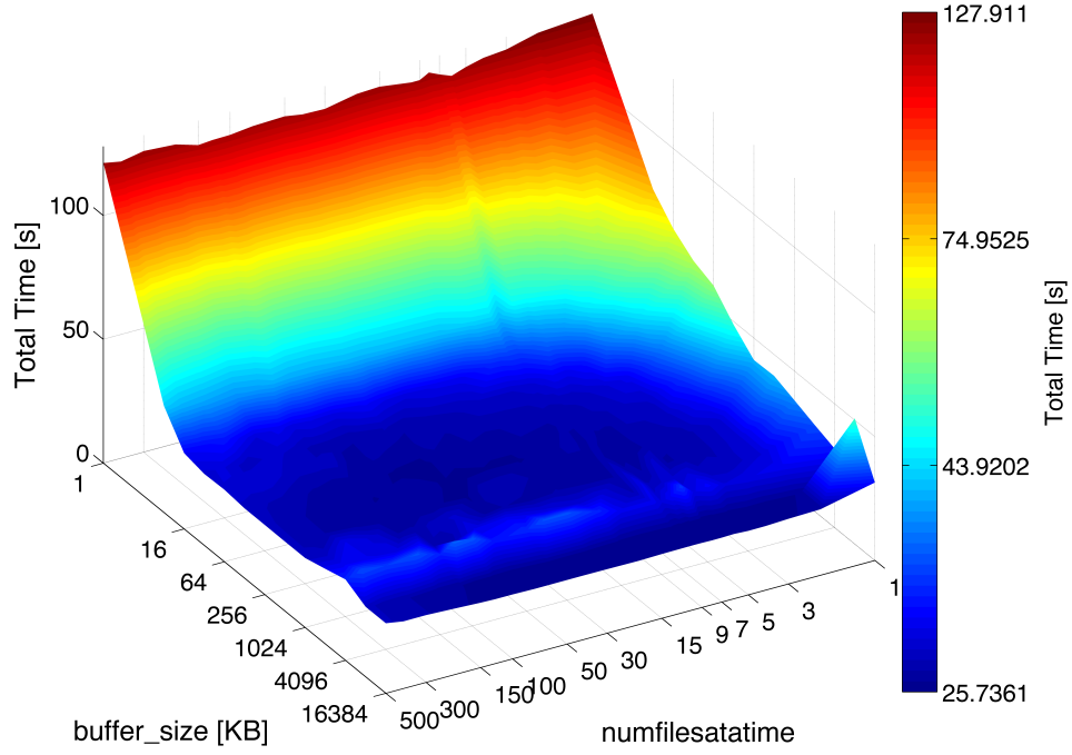
FIGURE 9. Testing Paramotopy run times versus internal parameters, using a 500000 parameter point sample, in the 9 \times 9 Duffing system. The horizontal axes are logarithmic, with linear vertical axis corresponding to run time. Coloration is logarithmic in runtime. Optimal settings are bounded away from the origin.
