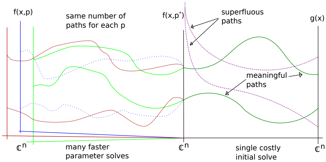
FIGURE 2. An illustration of the Paramotopy method. Starting at the right from a constructed system in Bertini, we continue to the left, to solutions of the desired system for random complex values. From there, we continue once more (many times more) to any desired set of parameter values.
