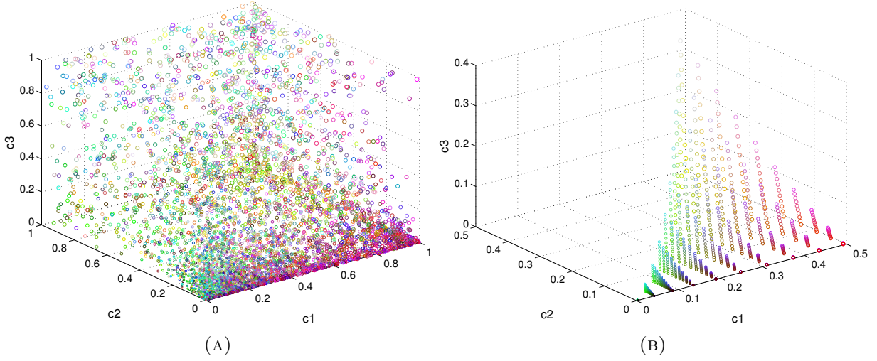
FIGURE 14. Chemical equilibria solution plots for Craciun Helton Williams Example 2.3. Colors of points are determined by letting the RGB value be determined by normalized values of (d1, d2, d3) . Hence, the red colored points are heavy in d1 , whereas green are heavy in d2 , etc.
