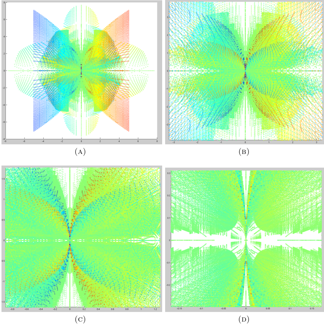
FIGURE 5. Successive zooms into the origin of solution space. Points represent projection onto z_0, z_1 , with color determined by z_3 . All solutions for the entire scan through parameter space plotted.
