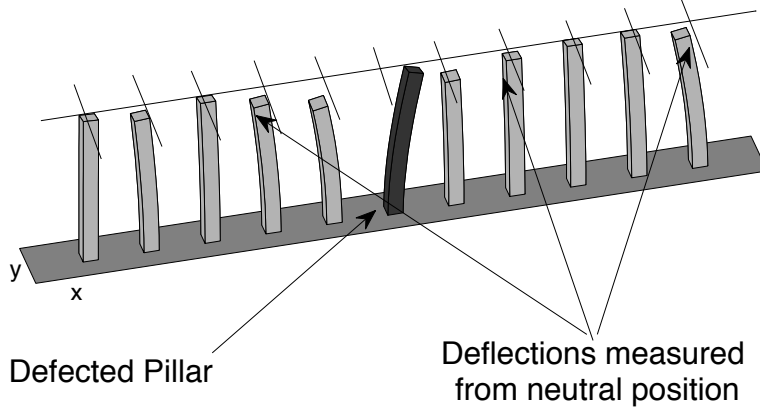
FIGURE 16. An illustration of one dimensional cantilever array that is able to undergo vibrations in two directions. Also drawn is a defected pillar that is used to pin the ILM appearing from random initial condition to that pillar.
