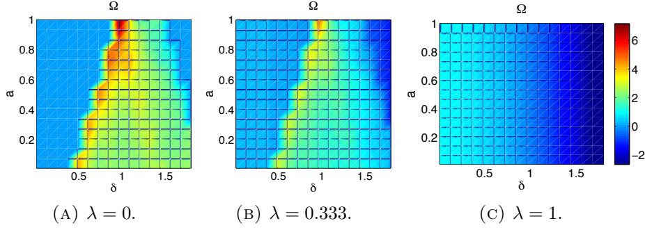
FIGURE 29. Considering grasping on the second link to restore workspace after failure of joint 2 of a PUMA robot. a) Measurement of the intersection workspace |W_{\cap}| , as a function of \delta . b)-c) Contours of the objective function \Omega versus (\delta, a) for 3D cooperating robots. Note that for the case a), \lambda = 0 and the objective function \Omega is equal to the measure of post-failure workspace |W_f| .
