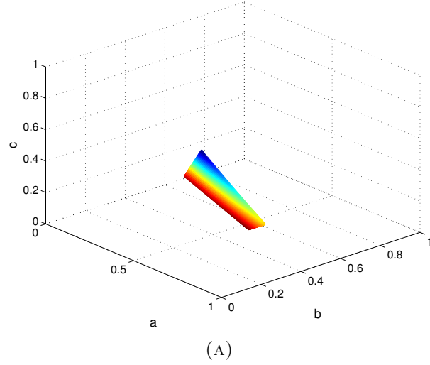
FIGURE 15. Solution Plot for Craciun, Helton, Williams Example 6.1. This five-variable, 13-parameter system has a unique positive equilibrium for each parameter point. Here, we have projected onto coordinates (a, b, c) , with coloring coming from \sqrt{p^2 + q^2} .
