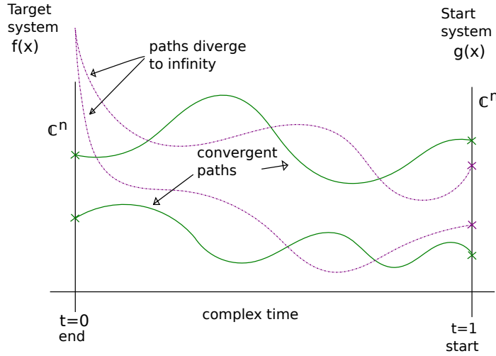
FIGURE 1. An illustration of generic homotopy continuation. The magenta paths from the constructed start system diverge to \infty , while green paths converge to solutions to the desired system f . Theory guarantees that off a set of measure zero in \mathbb{C}^n , we will have a uniform number of (complex) solutions to f . The divergent paths are present because the constructed start system has a surplus of solutions.
