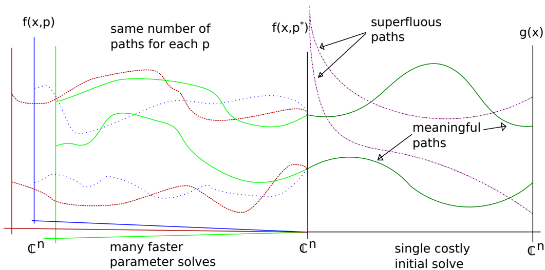
FIGURE 31. Parameter Homotopy, with initial ‘Step1’ run.
