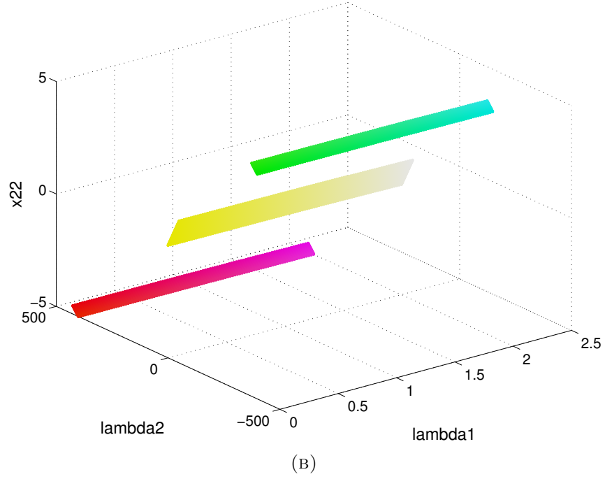
FIGURE 6. Solution plots for the Duffing 9 \times 9 system. (a) Projections onto variables \lambda_1 , \lambda_2 , x_{22} , with points colored according to the corresponding value of \sqrt{x_{11}^2 + x_{21}^2} . (b) The same coordinate projections, with coloring coming by letting RGB values be set according to normalized values of \mu_3 , \mu_4 , x_{12} .
