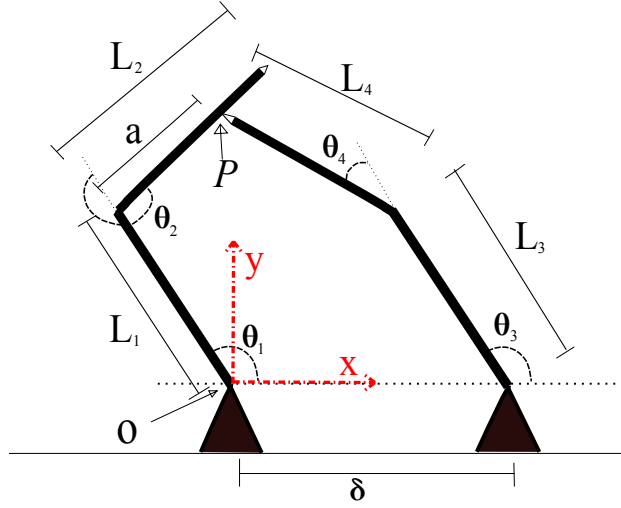
FIGURE 24. Two robots in grasping configuration, with functional robot contacting the disabled unit at point P . This is a simplified 2D model of the general 6D position and orientation scenario.
